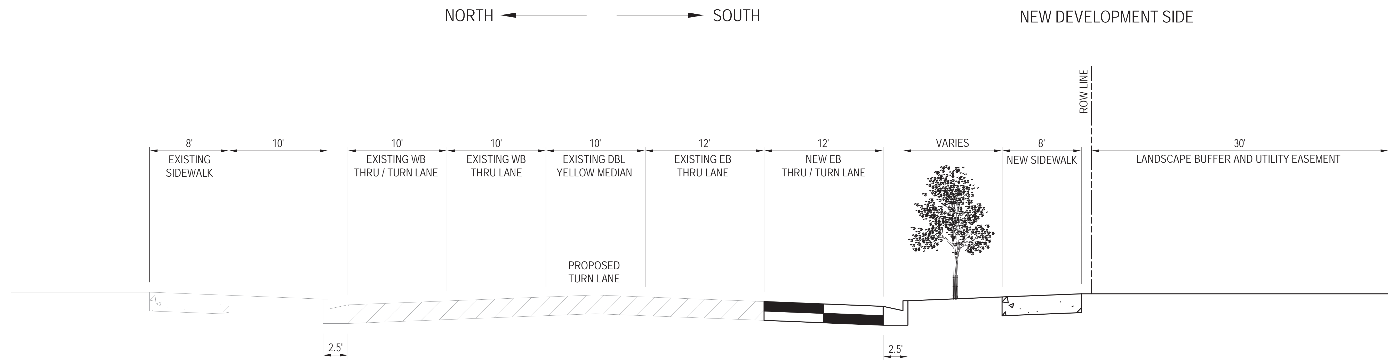
A ARAPAHOE ROAD IMPROVED SECTION NOT TO SCALE
